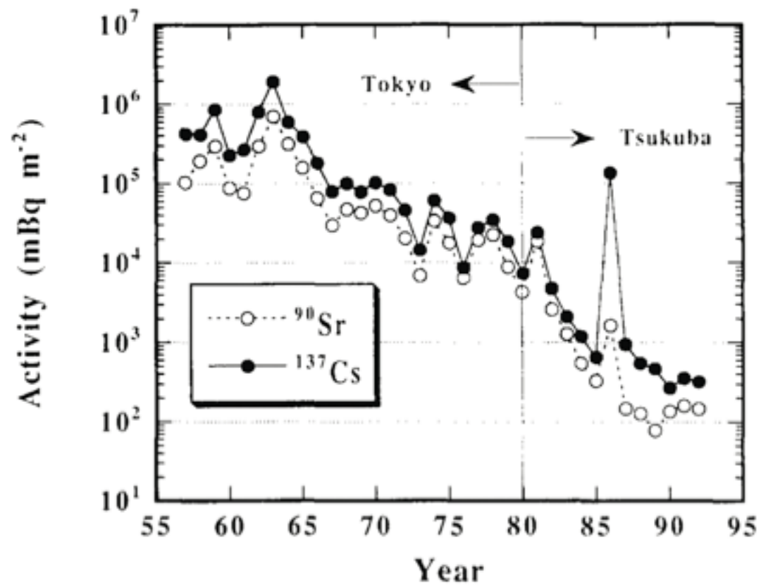
Fig. 1. Annual radioactivity deposition observed at MRI since 1957 (MRI moved to Tsukuba from Tokyo in 1980).
